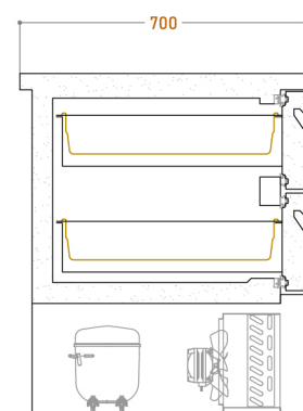
Section view
