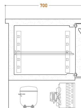
Section view
