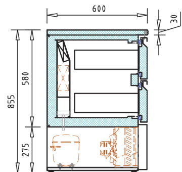
Section view
