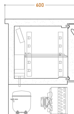
Section view
