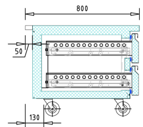
Section view
