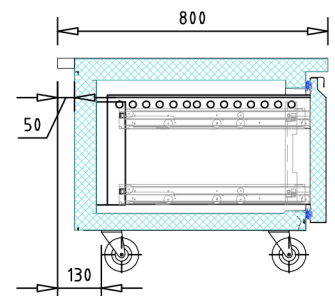
Section view
