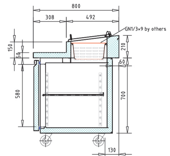
Section view
