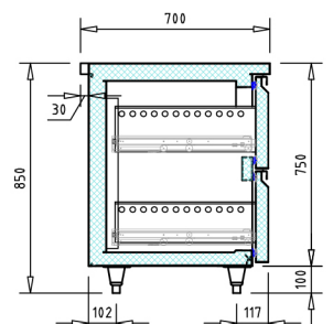
Section view
