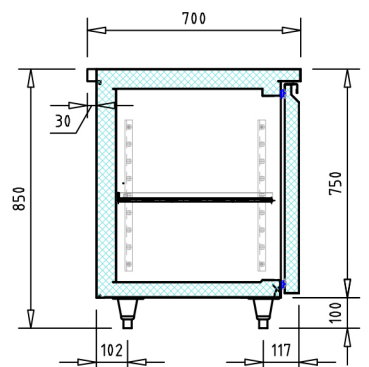
Section view
