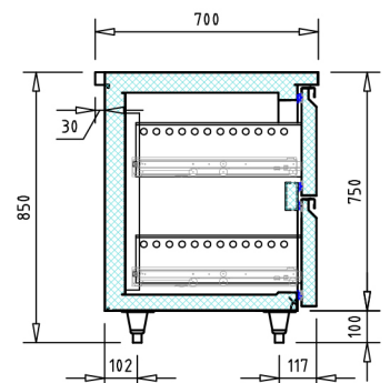
Section view
