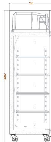
Section view
