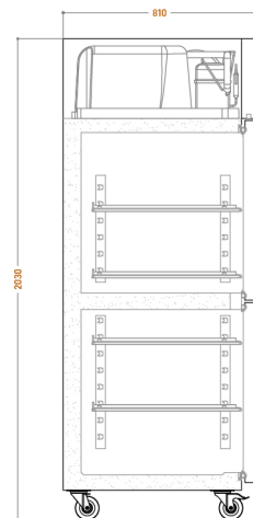
Section view
