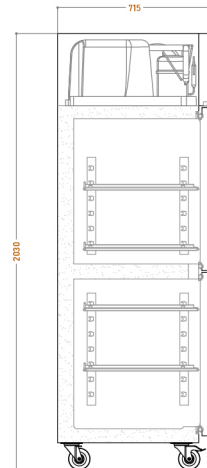
Section view
