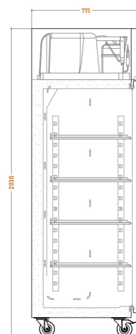
Section view
