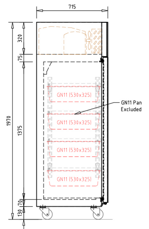
Section view
