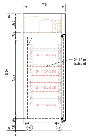
Section view
