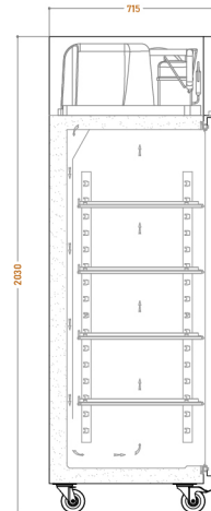
Section view
