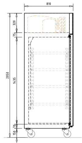
Section view
