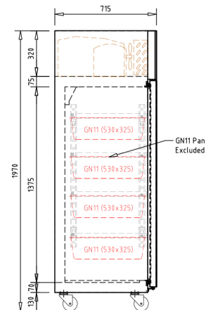
Section view
