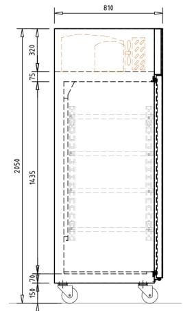
Section view
