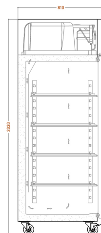
Section view
