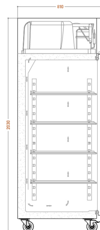
Section view
