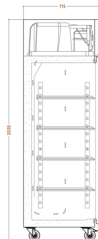
Section view
