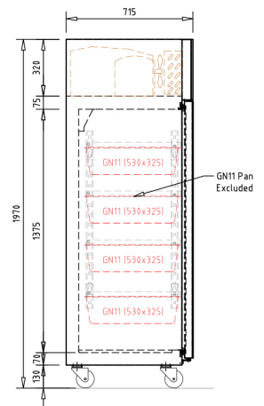
Section view
