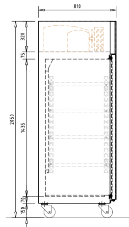
Section view
