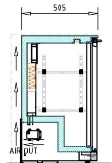
Section view
