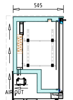
Section view
