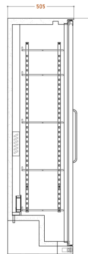
Section view
