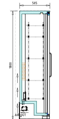
Section view
