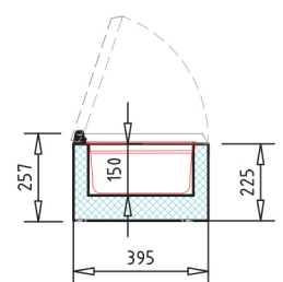
Section view
