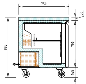
Section view
