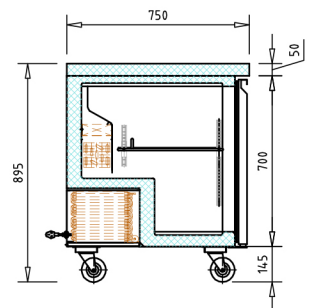
Section view
